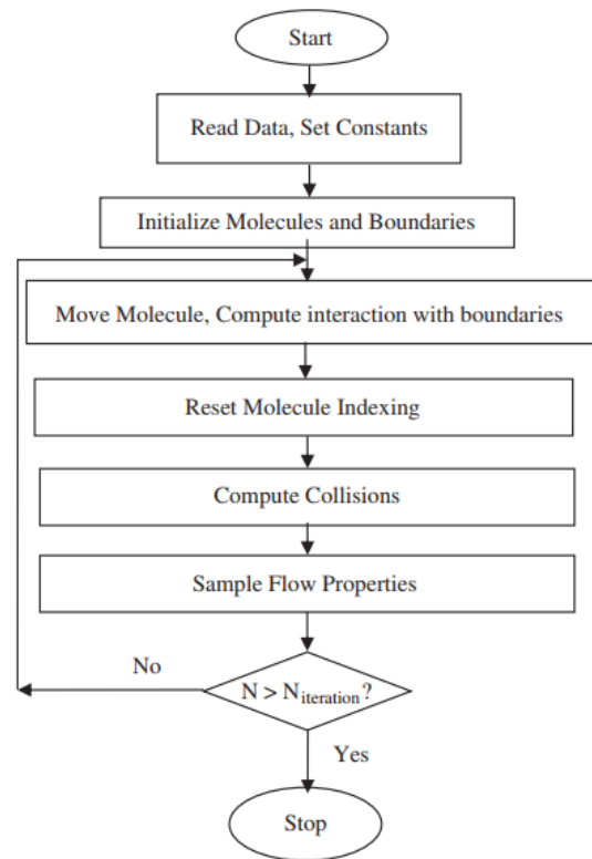
Fig. 1. Flowchart of the DSMC algorithm
