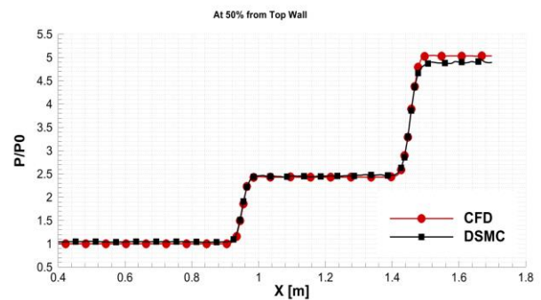
Fig. 5. Comparison of Pressure Ratio between CFD and DSMC results at the 50% distance from the Top Wall
