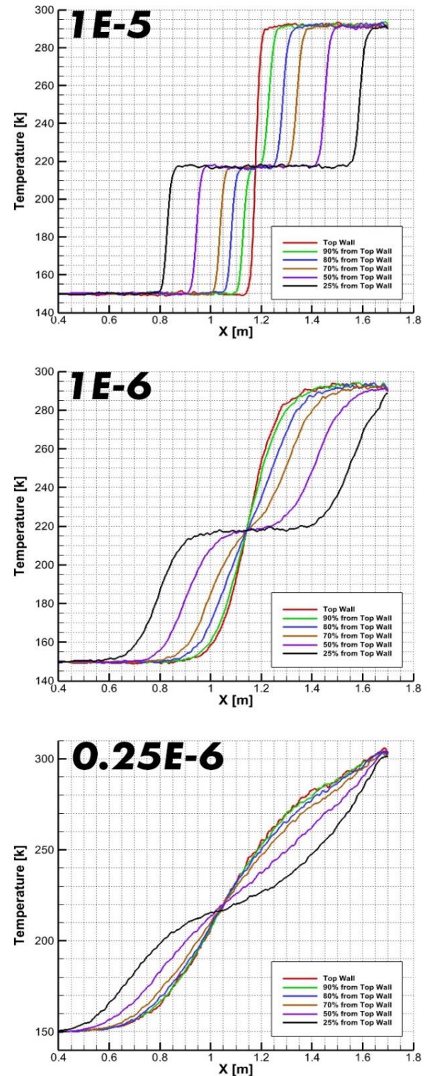
Fig. 8. Temperature distribution at different distances from the top wall
