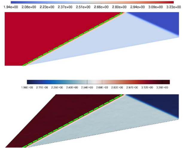
Fig. 4. Contours of Mach number obtained by CFD (upper) and DSMC (lower). The analytical solution is indicated by dashed lines.
