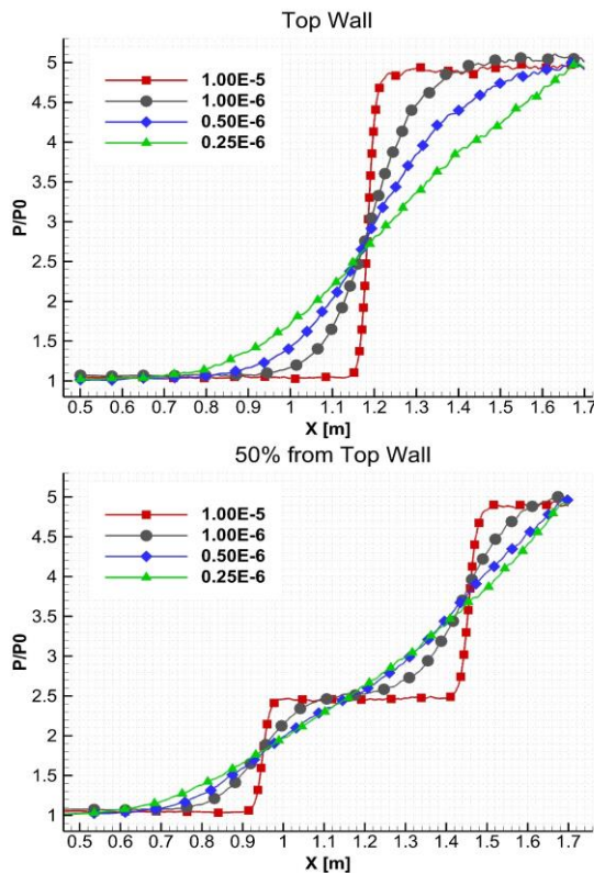
Fig. 9. Pressure ratio for different rarefaction levels at the top wall and 50% distance from the top wall
