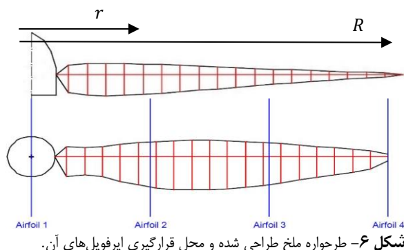
Fig. 6. Schematic of the designed propeller and the location of its airfoils.
